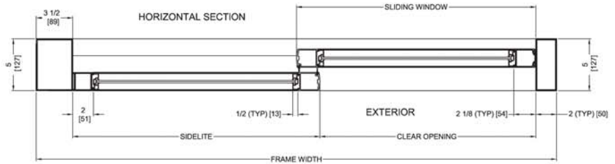
GT1500-01L-A, automatic single-slide window
